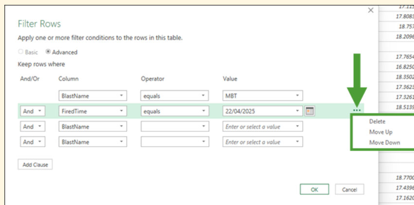
Figure 4-18 Deleting and reordering filtering conditions.
