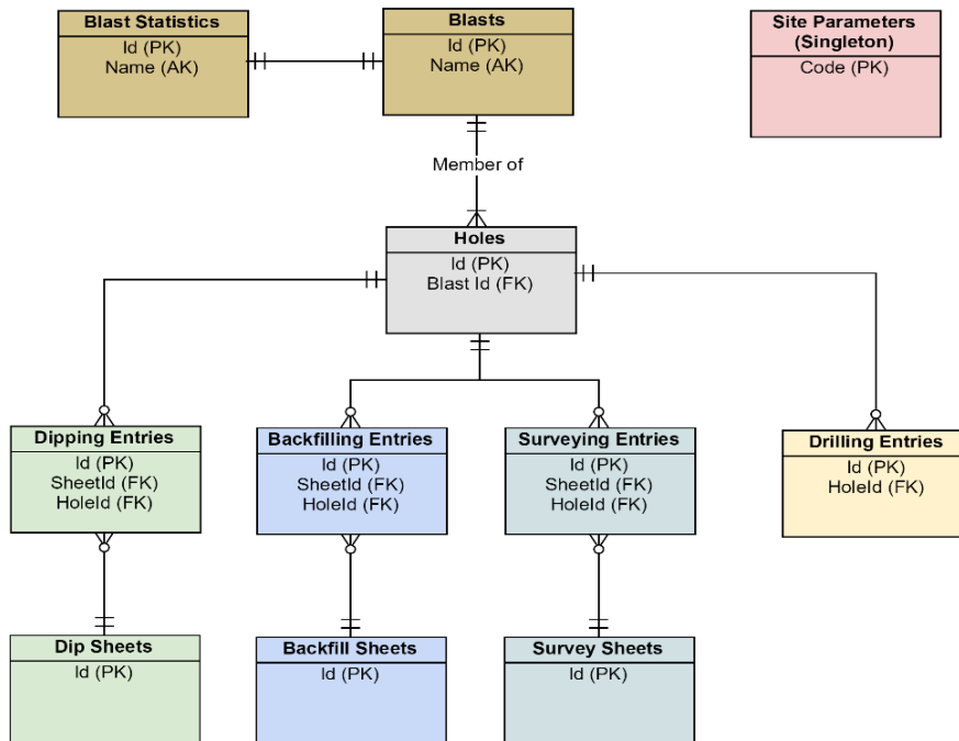
Figure 2-1 Entity relationship diagram (non-charging entities).
